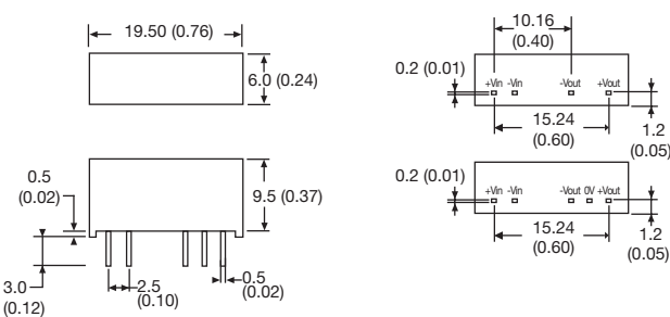
SIP package
