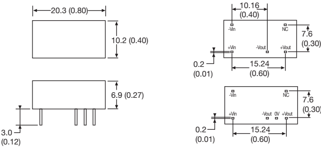
DIP package
