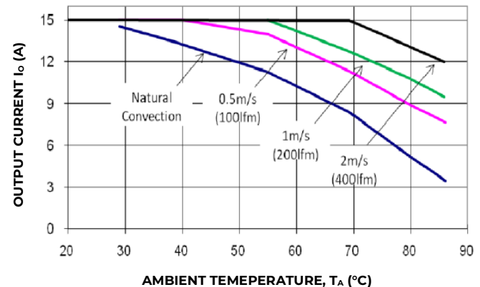
Figure 16. Output Current Derating for the Open Frame Module; Airflow in the Transverse Direction from V_{out}(-) to V_{out}(+) ; V_{IN} = 48V , V_O = 5.0V .
