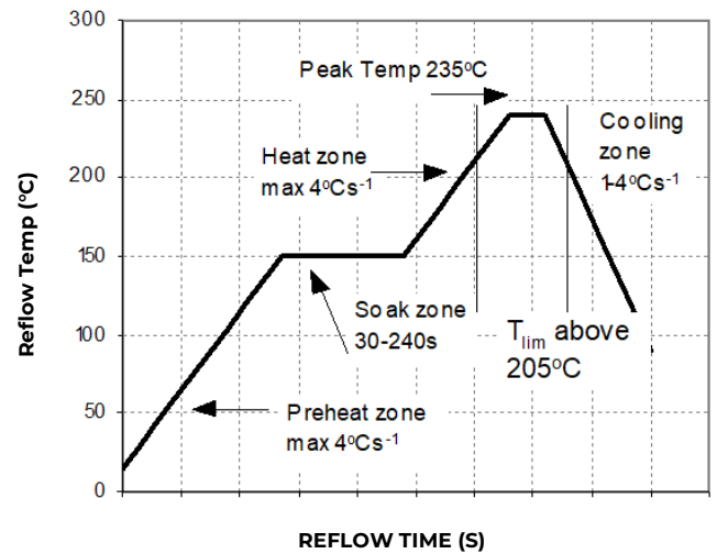
Figure 21. Reflow Profile for Tin/Lead (Sn/Pb) process.
