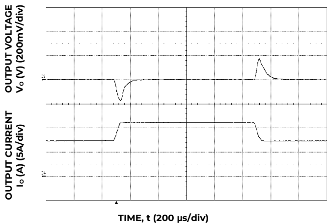
Figure 3. Transient Response to 0.1A/μS Dynamic Load Change from 50% to 75% to 50% of full load, V_{in}=48V , C_o>100\mu F .
