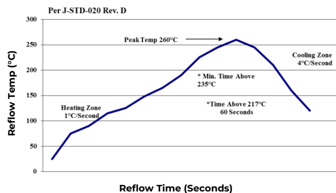
Figure 23. Recommended linear reflow profile using Sn/Ag/Cu solder.
