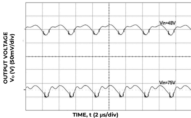
Figure 2. Typical output ripple and noise ( I_o = I_{o,max} ).
