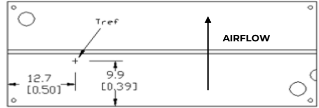
Figure 14. T_{ref} Temperature Measurement Location for Module with Heatplate.
