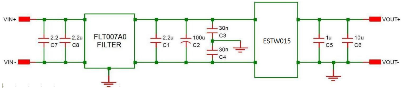
Figure 24. EMC Considerations
