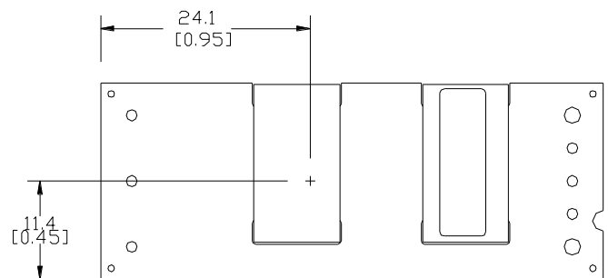
Figure 20. Pick and Place Location.
