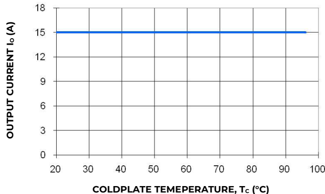
Figure 19. Derated Output Current versus Cold Wall Temperature with local ambient temperature around module at 85°C; V_{IN} = 48V .
