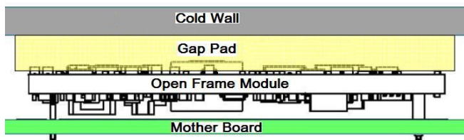
Figure 18. Cold Wall Mounting
