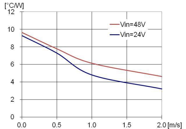
Figure 15. Thermal Resistance for the Open Frame Module; Airflow in the Transverse Direction from V_{out}(-) to V_{out}(+) ; V_{IN} = 48V , V_O = 5.0V .
