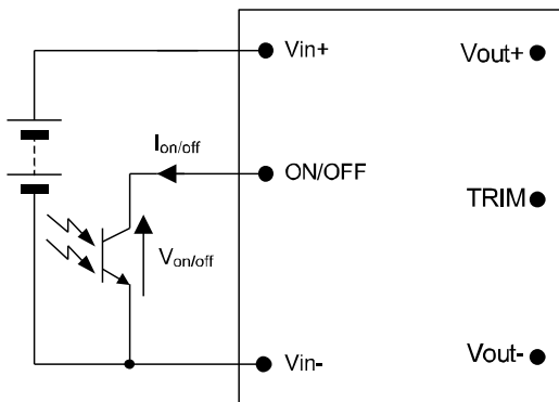
Figure 10. Remote On/Off Implementation.
