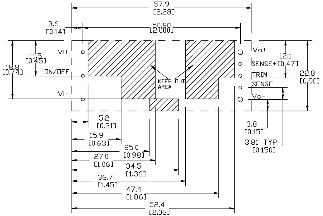
TH Recommended Pad Layout (Component Side View)
