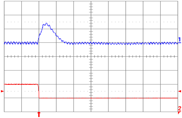
Fig. 2.0V.8: Output voltage response for V_{out} = 2.0\text{ V} to negative load current step change from 10 A to 5 A with slew rate of -5 A/ \mu\text{s} at V_{in} = 5\text{ V} . Top trace: output voltage (100 mV/div.); Bottom trace: load current (5 A/div.). C_o = 47\text{ }\mu\text{F} ceramic + 1 \mu\text{F} ceramic. Time scale: 20 \mu\text{s} /div.
