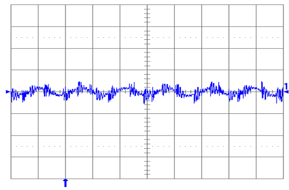
Fig. 2.0V.6: Output voltage ripple (20 mV/div.) at full rated load current into a resistive load with external capacitance 47 \mu\text{F} ceramic + 1 \mu\text{F} ceramic, and V_{in} = 5 V for V_{out} = 2.0 V. Time scale: 2 μs/div
