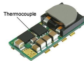
Fig. F: Location of the thermocouple for thermal testing.
