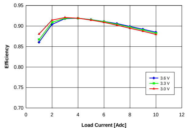
Fig. 1.2V.4: Efficiency vs. load current and input voltage for V_{out} = 1.2 V converter mounted horizontally with air flowing at a rate of 200 LFM (1 m/s) and T_a = 25 °C.
