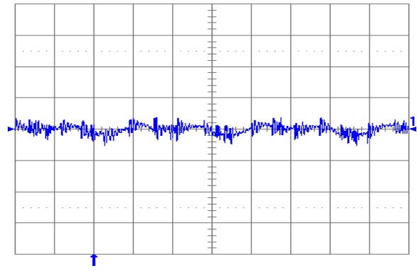
Fig. 1.0V.6: Output voltage ripple (20 mV/div.) at full rated load current into a resistive load with external capacitance 47\text{ }\mu\text{F} ceramic + 1\text{ }\mu\text{F} ceramic, and V_{in} = 5 V for V_{out} = 1.0 V. Time scale: 2\text{ }\mu\text{s/div.}
