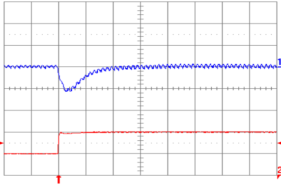
Fig. 2.0V.7: Output voltage response for V_{out} = 2.0\text{ V} to positive load current step change from 5 A to 10 A with slew rate of 5 A/ \mu\text{s} at V_{in} = 5\text{ V} . Top trace: output voltage (100 mV/div.); Bottom trace: load current (5 A/div.). C_o = 47\text{ }\mu\text{F} ceramic + 1 \mu\text{F} ceramic. Time scale: 20 \mu\text{s} /div.
