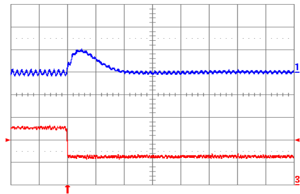
Fig. 1.0V.8: Output voltage response for V_{out} = 1.0 V to negative load current step change from 10 A to 5 A with slew rate of -5\text{ A}/\mu\text{s} at V_{in} = 5 V. Top trace: output voltage (100 mV/div.); Bottom trace: load current (5 A/div.). C_o = 47\text{ }\mu\text{F} ceramic + 1\text{ }\mu\text{F} ceramic. Time scale: 20\text{ }\mu\text{s/div.}
