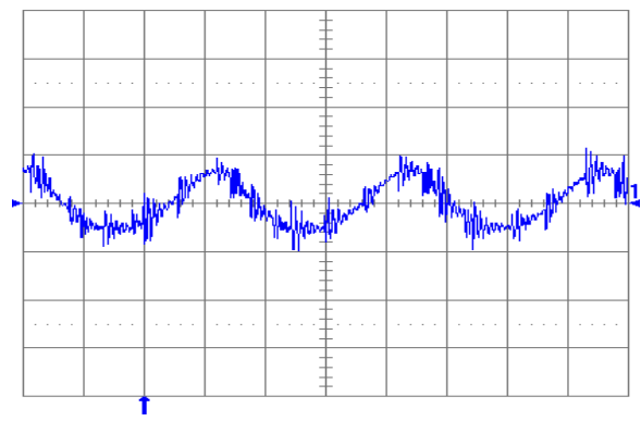
Fig. 3.3V.6: Output voltage ripple (20 mV/div.) at full rated load current into a resistive load with external capacitance 47 \mu\text{F} ceramic + 1 \mu\text{F} ceramic, and V_{in} = 5 V for V_{out} = 3.3 V. Time scale: 2 μs/div.
