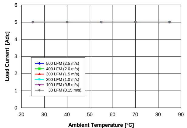
Fig. 1.0V.2: Available load current vs. ambient temperature and airflow rates for V_{out} = 1.0V converter mounted horizontally with V_{in} = 12V , air flowing from pin 5 to pin 1 and maximum MOSFET temperature \leq 120^\circ C .
