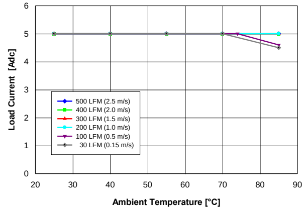
Fig. 5.0V.2: Available load current vs. ambient temperature and airflow rates for V_{out} = 5.0V converter mounted horizontally with V_{in} = 12V , air flowing from pin 5 to pin 1 and maximum MOSFET temperature \leq 120^{\circ}C .
