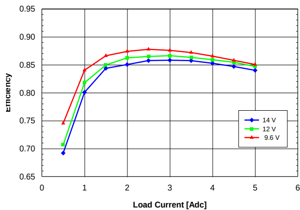
Fig. 2.0V.3: Efficiency vs. load current and input voltage for V_{out} = 2.0V converter mounted vertically with air flowing from pin 5 to pin 1 at a rate of 200 LFM (1 m/s) and T_a = 25\text{ }^{\circ}C .
