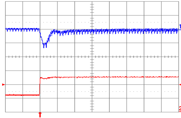
Fig. 1.2V.6: Output voltage response for V_{out} = 1.2V to a positive load current step change from 2.5A to 5A with a slew rate of 5A/\mu s at V_{in} = 12V . Top trace: output voltage (100mV/div); Bottom trace: load current (2A/div). C_o = 47\mu F ceramic. Time scale: 20 \mu s/div .
