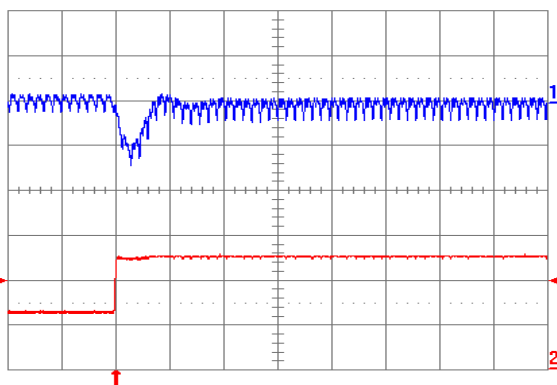
Fig. 2.5V.7: Output voltage response for V_{out} = 2.5V to a positive load current step change from 2.5A to 5A with a slew rate of 5A/\mu s at V_{in} = 12V . Top trace: output voltage (100mv/div); Bottom trace: load current (2A/div). C_o = 47\mu F ceramic. Time scale: 20 \mu s /div.
