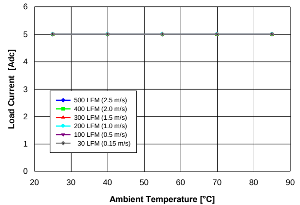
Fig. 2.0V.2: Available load current vs. ambient temperature and airflow rates for V_{out} = 2.0V converter mounted horizontally with V_{in} = 12V , air flowing from pin 5 to pin 1 and maximum MOSFET temperature \leq 120\text{ }^{\circ}C .
