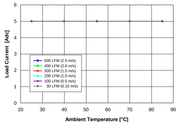
Fig. 2.5V.2: Available load current vs. ambient temperature and airflow rates for V_{out} = 2.5V converter mounted horizontally with V_{in} = 12V , air flowing from pin 5 to pin 1 and maximum MOSFET temperature \leq 120^\circ C .
