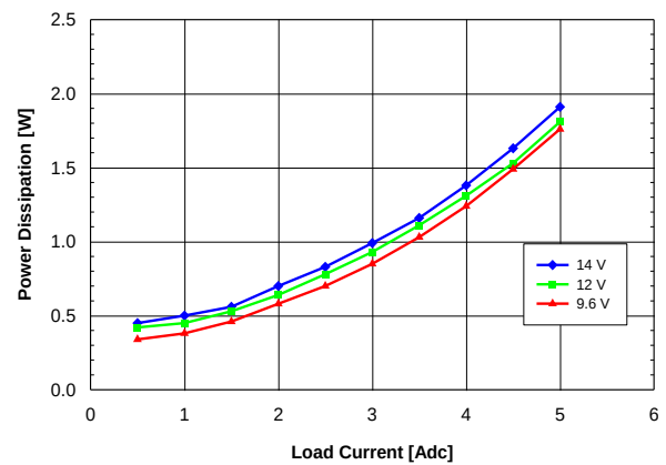
Fig. 2.0V.4: Power Loss vs. load current and input voltage for V_{out} = 2.0V converter mounted vertically with air flowing from pin 5 to pin 1 at a rate of 200 LFM (1 m/s) and T_a = 25\text{ }^{\circ}C .
