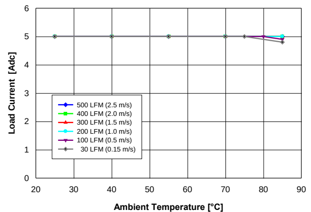
Fig. 3.3V.2: Available load current vs. ambient temperature and airflow rates for V_{out} = 3.3V converter mounted horizontally with V_{in} = 12V , air flowing from pin 5 to pin 1 and maximum MOSFET temperature \leq 120^\circ C .
