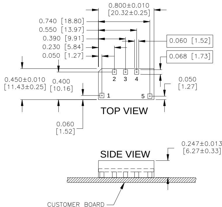
YM12S Pinout (Surface Mount)
