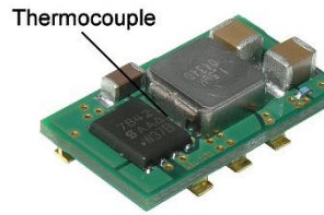
Fig. C: Location of the thermocouple for thermal testing
