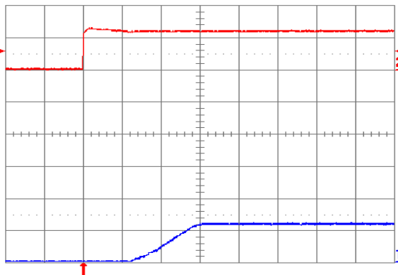
Fig. 1.2V.5: Turn-on transient for V_{out} = 1.2V with application of V_{in} = 12V at full rated load current (resistive) and 47\mu F external capacitance. Top trace: V_{in} (10V/div); Bottom trace: V_{out} (1V/div); Time scale: 2 ms/div.
