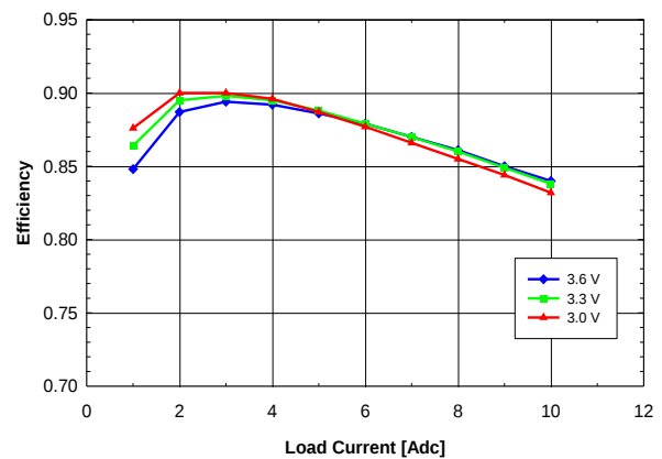
Fig. 0.7525V.4: Efficiency vs. load current and input voltage for V_{out} = 0.7525V converter mounted horizontally with air flowing from pin 10 to pin 1 at a rate of 200 LFM (1m/s) and T_a = 25^\circ C .
