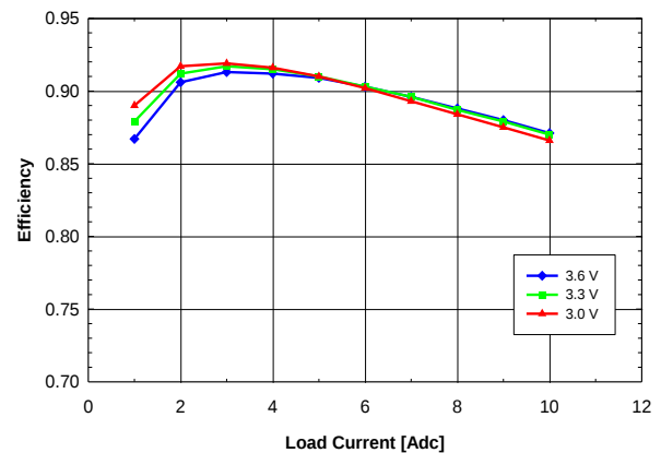
Fig. 1.0V.4: Efficiency vs. load current and input voltage for V_{out} = 1.0V converter mounted horizontally with air flowing from pin 10 to pin 1 at a rate of 200 LFM (1m/s) and T_a = 25^{\circ}C .
