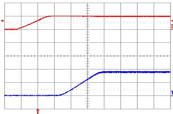
Fig. 1.8V.5: Turn-on transient for V_{out} = 1.8 V with application of V_{in} at full rated load current (resistive) and 47 \mu F external capacitance at V_{in} = 5 V. Top trace: V_{in} (5 V/div.); Bottom trace: output voltage (1 V/div.); Time scale: 2 ms/div.
