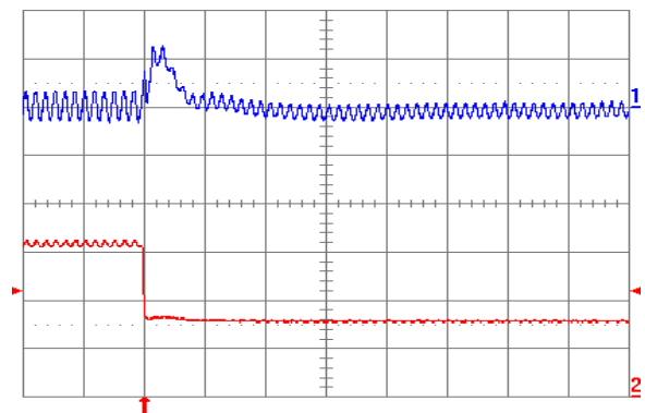
Fig. 2.0V.8: Output voltage response for V_{out} = 2.0 V to negative load current step change from 5 A to 2.5 A with slew rate of -5 A/ \mu\text{s} at V_{in} = 5 V. Top trace: output voltage (100 mV/div.); Bottom trace: load current (2 A/div.). C_o = 47 \mu\text{F} ceramic + 1 \mu\text{F} ceramic. Time scale: 20 \mu\text{s} /div.
