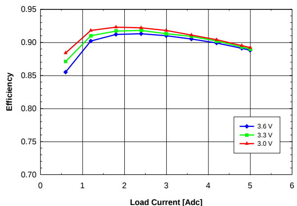
Fig. 1.5V.4: Efficiency vs. load current and input voltage for V_{out} = 1.5V converter mounted horizontally with air flowing from pin 5 to pin 1 at a rate of 200 LFM (1 m/s) and T_a = 25^\circ C .
