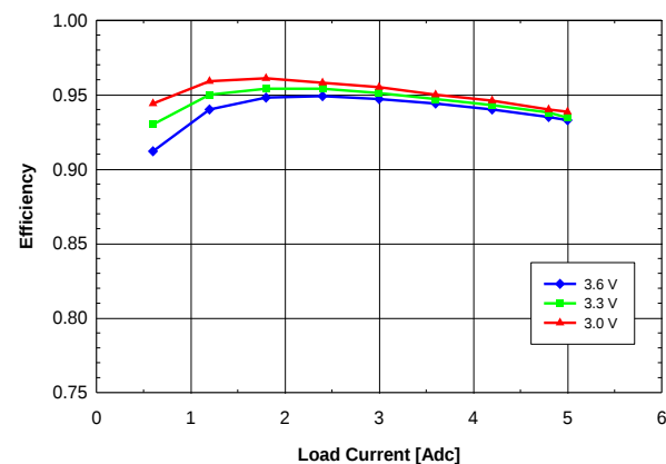
Fig. 2.5V.4: Efficiency vs. load current and input voltage for V_{out} = 2.5\text{ V} converter mounted vertically with air flowing from pin 5 to pin 1 at a rate of 200 LFM (1 m/s) and T_a = 25\text{ }^{\circ}\text{C} .
