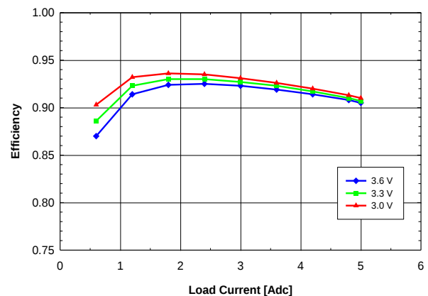
Fig. 1.8V.4: Efficiency vs. load current and input voltage for V_{out} = 1.8 V converter mounted horizontally with air flowing from pin 5 to pin 1 at a rate of 200 LFM (1 m/s) and T_a = 25 °C.
