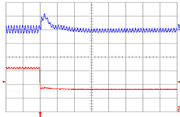
Fig. 1.5V.8: Output voltage response for V_{out} = 1.5 V to negative load current step change from 5 A to 2.5 A with slew rate of -5 A/ \mu s at V_{in} = 5 V. Top trace: output voltage (100 mV/div.); Bottom trace: load current (2 A/div.). C_o = 47 \mu F ceramic + 1 \mu F ceramic. Time scale: 20 \mu s/div.
