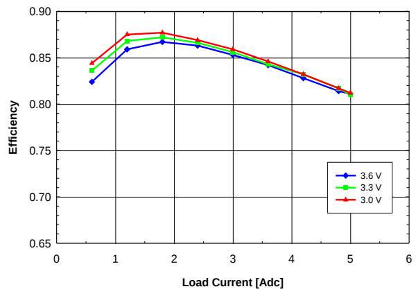
Fig. 0.7525V.4: Efficiency vs. load current and input voltage for V_{out} = 0.7525\text{ V} converter mounted vertically with air flowing from pin 5 to pin 1 at a rate of 200 LFM (1 m/s) and T_a = 25\text{ }^{\circ}\text{C} .
