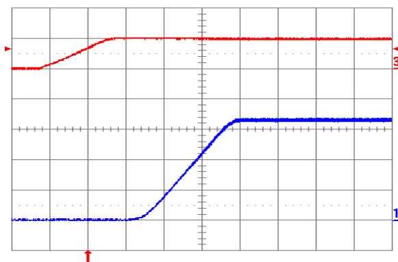
Fig. 3.3V.5: Turn-on transient for V_{out} = 3.3 V with application of V_{in} at full rated load current (resistive) and 47 \mu F external capacitance at V_{in} = 5 V. Top trace: V_{in} (5 V/div.); Bottom trace: output voltage (1V/div.); Time scale: 2 ms/div.
