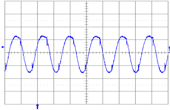
Fig. 2.5V.5: Output voltage ripple ( 20\text{ mV/div.} ) at full rated load current into a resistive load with external capacitance 10\text{ }\mu\text{F} ceramic + 1\text{ }\mu\text{F} ceramic and V_{in} = 5\text{ V} for V_{out} = 2.5\text{ V} . Time scale: 2\text{ }\mu\text{s/div.}
