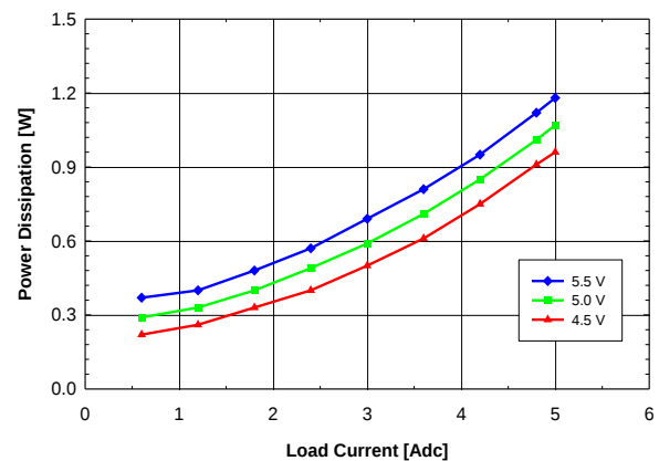
Fig. 3.3V.4: Power Loss vs. load current and input voltage for V_{out} = 3.3 V converter mounted vertically with air flowing from pin 5 to pin 1 at a rate of 200 LFM (1 m/s) and T_a = 25 °C.
