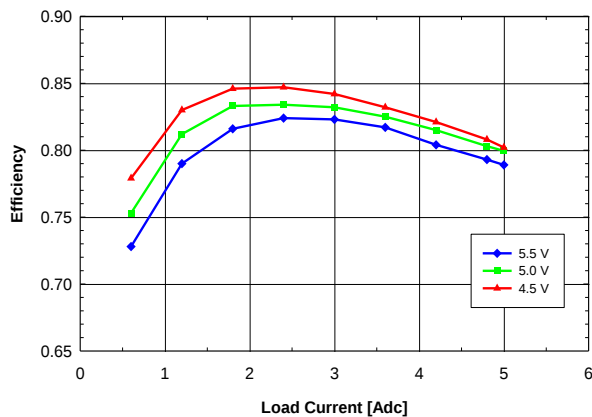
Fig. 0.7525V.3: Efficiency vs. load current and input voltage for V_{out} = 0.7525\text{ V} converter mounted vertically with air flowing from pin 5 to pin 1 at a rate of 200 LFM (1 m/s) and T_a = 25\text{ }^{\circ}\text{C} .
