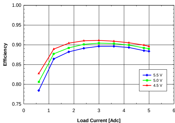
Fig. 1.8V.3: Efficiency vs. load current and input voltage for V_{out} = 1.8 V converter mounted vertically with air flowing from pin 5 to pin 1 at a rate of 200 LFM (1 m/s) and T_a = 25 °C.
