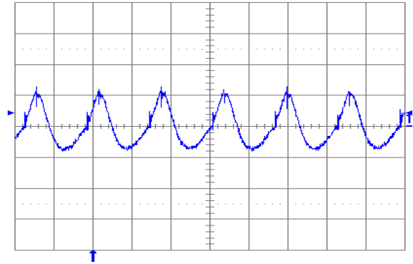
Fig. 0.7525V.5: Output voltage ripple (20 mV/div.) at full rated load current into a resistive load with external capacitance 10 \mu F ceramic + 1 \mu F ceramic and V_{in} = 5 V for V_{out} = 0.7525 V. Time scale: 2 \mu s/div.
