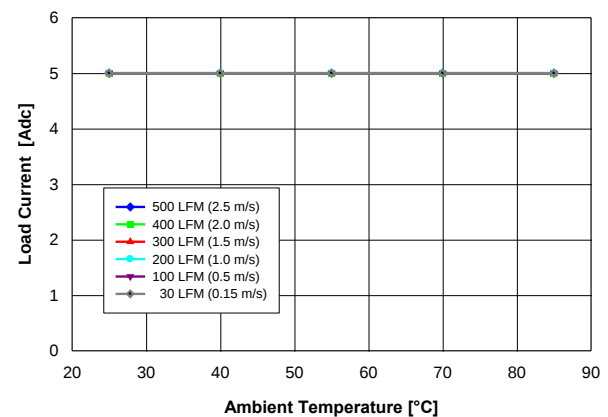
Fig. 1.2V.2: Available load current vs. ambient temperature and airflow rates for V_{out} = 1.2 V converter mounted horizontally with V_{in} = 5 V, air flowing from pin 5 to pin 1 and maximum MOSFET temperature \leq 120 °C.
