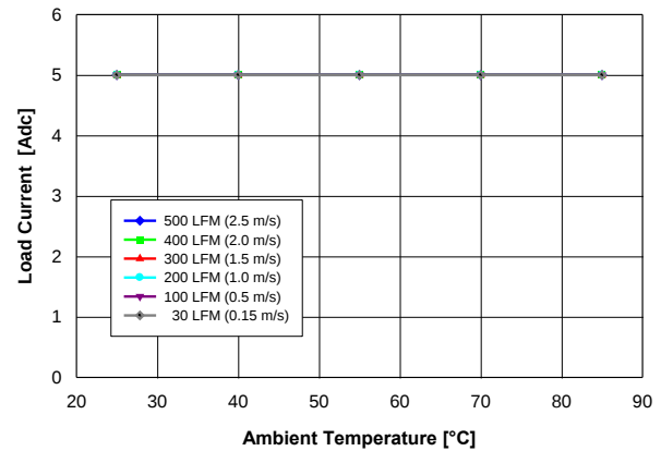
Fig. 3.3V.2: Available load current vs. ambient temperature and airflow rates for V_{out} = 3.3 V converter mounted horizontally with V_{in} = 5 V, air flowing from pin 5 to pin 1 and maximum MOSFET temperature \leq 120 °C.
