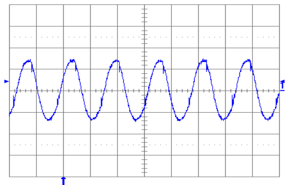
Fig. 1.8V.6: Output voltage ripple (20 mV/div.) at full rated load current into a resistive load with external capacitance 10 \mu F ceramic + 1 \mu F ceramic and V_{in} = 5 V for V_{out} = 1.8 V. Time scale: 2 \mu s/div.
