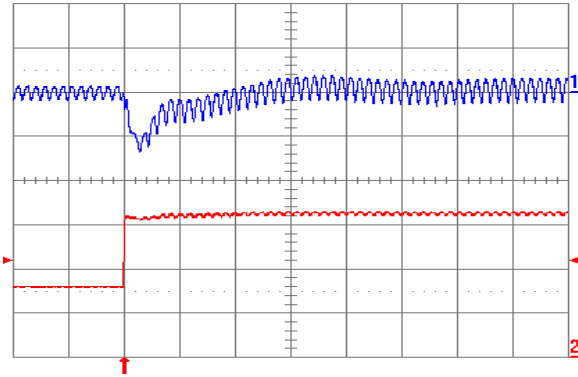
Fig. 3.3V.7: Output voltage response for V_{out} = 3.3\text{ V} to positive load current step change from 2.5 A to 5 A with slew rate of 5\text{ A}/\mu\text{s} at V_{in} = 5\text{ V} . Top trace: output voltage (100 mV/div.); Bottom trace: load current (2 A/div.). C_o = 47\text{ }\mu\text{F} ceramic + 1\text{ }\mu\text{F} ceramic. Time scale: 20\text{ }\mu\text{s}/\text{div} .
