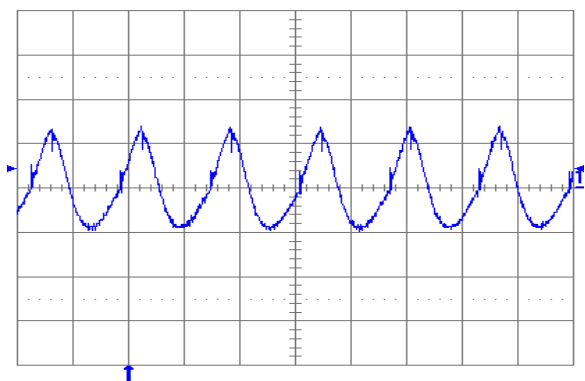
Fig. 1.0V.6: Output voltage ripple (20 mV/div.) at full rated load current into a resistive load with external capacitance 10 \mu\text{F} ceramic + 1 \mu\text{F} ceramic and V_{in} = 5 V for V_{out} = 1.0 V. Time scale: 2 μs/div.
