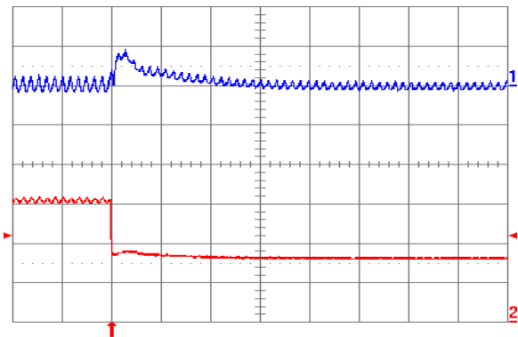
Fig. 0.7525V.8: Output voltage response for V_{out} = 0.7525 V to negative load current step change from 5 A to 2.5 A with slew rate of -5 A/ \mu s at V_{in} = 5 V. Top trace: output voltage (100 mV/div.); Bottom trace: load current (2 A/div.). C_o = 47 \mu F ceramic + 1 \mu F ceramic. Time scale: 20 \mu s/div.
