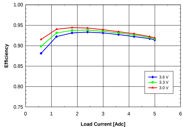
Fig. 2.0V.4: Efficiency vs. load current and input voltage for V_{out} = 2.0 V converter mounted vertically with air flowing from pin 5 to pin 1 at a rate of 200 LFM (1 m/s) and T_a = 25^\circ\text{C} .
