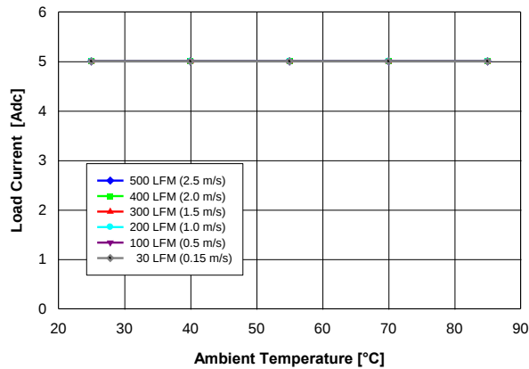
Fig. 3.3V.1: Available load current vs. ambient temperature and airflow rates for V_{out} = 3.3 V converter mounted vertically with V_{in} = 5 V, air flowing from pin 5 to pin 1 and maximum MOSFET temperature \leq 120 °C.
