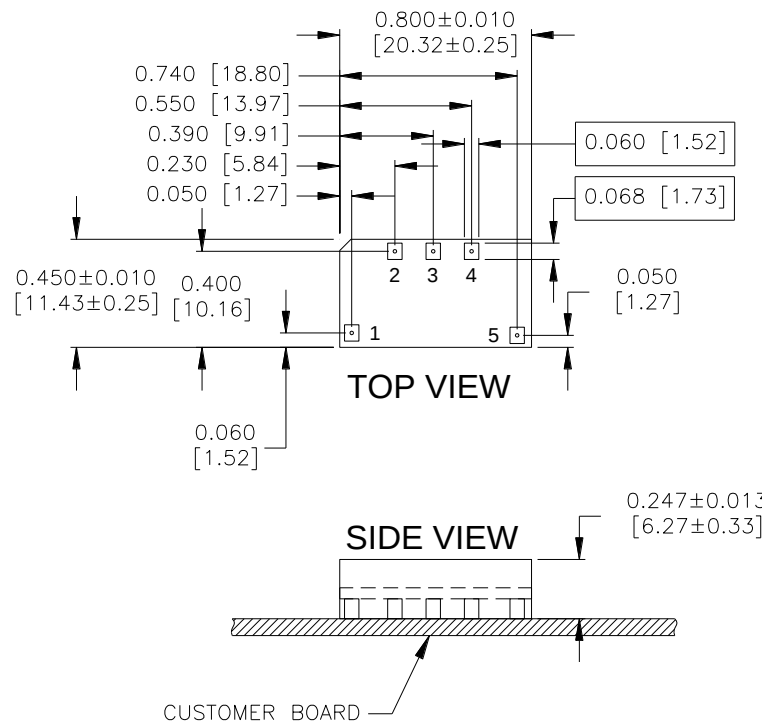
YM05S Pinout (Surface Mount)
