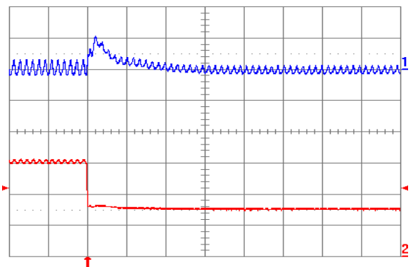
Fig. 1.2V.8: Output voltage response for V_{out} = 1.2 V to negative load current step change from 5 A to 2.5 A with slew rate of -5 A/ \mu s at V_{in} = 5 V. Top trace: output voltage (100 mV/div.); Bottom trace: load current (2 A/div.). C_o = 47 \mu F ceramic + 1 \mu F ceramic. Time scale: 20 \mu s/div.
