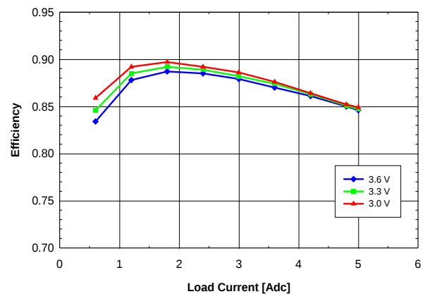
Fig. 1.0V.4: Efficiency vs. load current and input voltage for V_{out} = 1.0 V converter mounted vertically with air flowing from pin 5 to pin 1 at a rate of 200 LFM (1m/s) and T_a = 25 °C.
