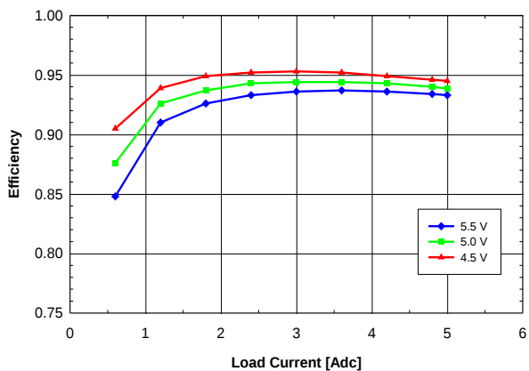
Fig. 3.3V.3: Efficiency vs. load current and input voltage for V_{out} = 3.3 V converter mounted vertically with air flowing from pin 5 to pin 1 at a rate of 200 LFM (1 m/s) and T_a = 25 °C.
