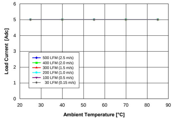
Fig. 1.8V.2: Available load current vs. ambient temperature and airflow rates for V_{out} = 1.8 V converter mounted horizontally with V_{in} = 5 V, air flowing from pin 5 to pin 1 and maximum MOSFET temperature \leq 120 °C.
