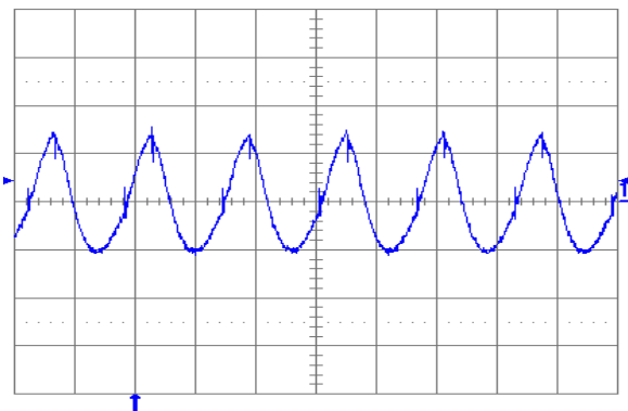
Fig. 1.2V.6: Output voltage ripple (20 mV/div.) at full rated load current into a resistive load with external capacitance 10 \mu F ceramic + 1 \mu F ceramic and V_{in} = 5 V for V_{out} = 1.2 V. Time scale: 2 \mu s/div.
