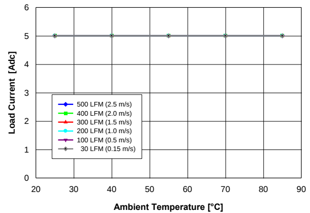
Fig. 0.7525V.2: Available load current vs. ambient temperature and airflow rates for V_{out} = 0.7525\text{ V} converter mounted horizontally with V_{in} = 5\text{ V} , air flowing from pin 5 to pin 1 and maximum MOSFET temperature \leq 120\text{ }^{\circ}\text{C} .
