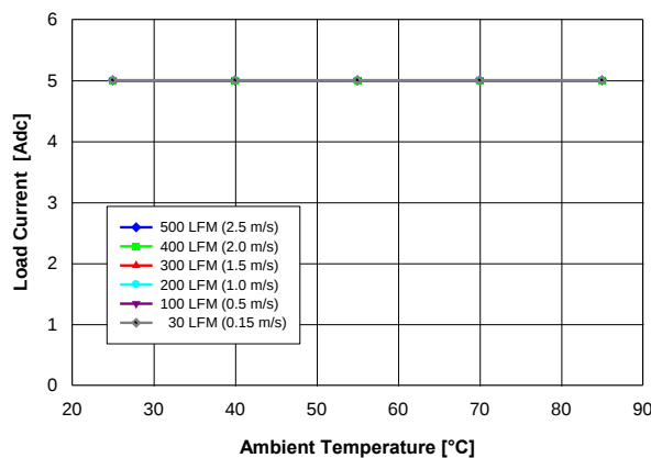
Fig. 1.2V.1: Available load current vs. ambient temperature and airflow rates for V_{out} = 1.2 V converter mounted vertically with V_{in} = 5 V, air flowing from pin 5 to pin 1 and maximum MOSFET temperature \leq 120 °C.
