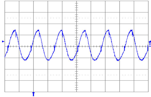
Fig. 1.5V.6: Output voltage ripple (20 mV/div.) at full rated load current into a resistive load with external capacitance 10 \mu F ceramic + 1 \mu F ceramic and V_{in} = 5 V for V_{out} = 1.5 V. Time scale: 2 \mu s/div.
