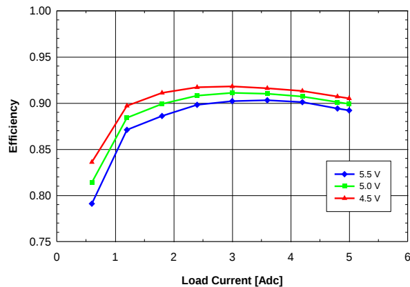
Fig. 2.0V.3: Efficiency vs. load current and input voltage for V_{out} = 2.0 V converter mounted vertically with air flowing from pin 5 to pin 1 at a rate of 200 LFM (1 m/s) and T_a = 25^\circ\text{C} .
