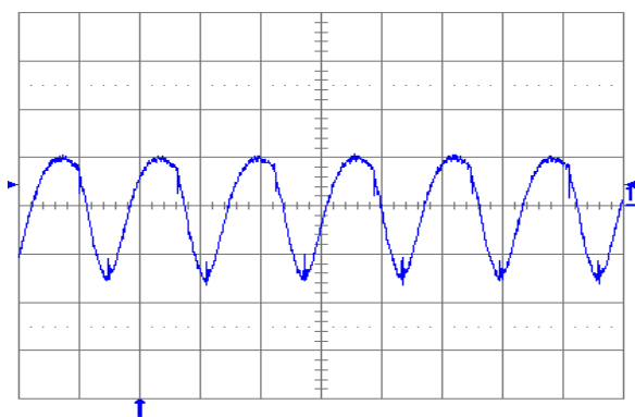
Fig. 3.3V.6: Output voltage ripple (20 mV/div.) at full rated load current into a resistive load with external capacitance 10 \mu F ceramic + 1 \mu F ceramic and V_{in} = 5 V for V_{out} = 3.3 V. Time scale: 2 \mu s/div.
