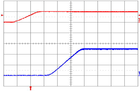
Fig. 2.5V.4: Turn-on transient for V_{out} = 2.5\text{ V} with application of V_{in} at full rated load current (resistive) and 47\text{ }\mu\text{F} external capacitance at V_{in} = 5\text{ V} . Top trace: V_{in} ( 5\text{ V/div.} ); Bottom trace: output voltage ( 1\text{ V/div.} ); Time scale: 2\text{ ms/div.}
