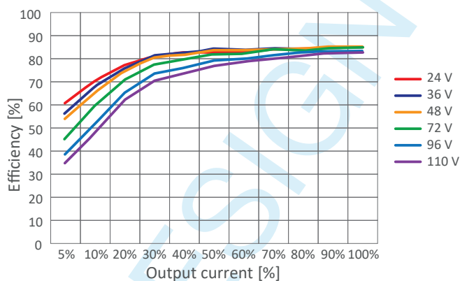
Figure 2. Efficiency vs. Output Load
