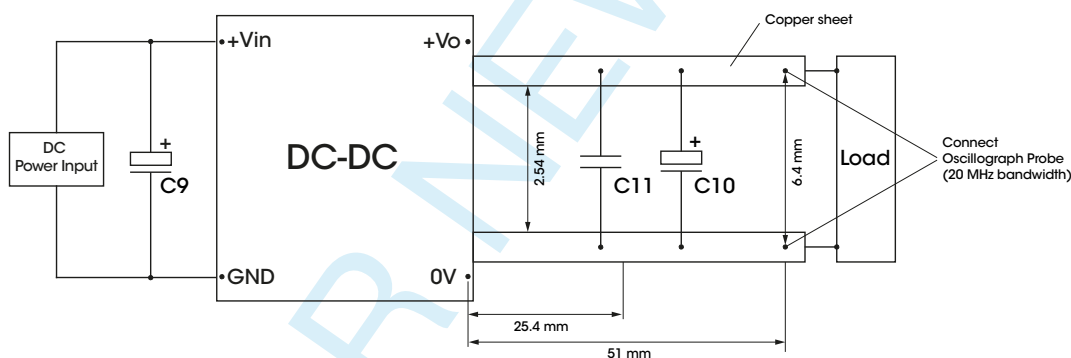
Figure 3. Recommended Test Circuit
