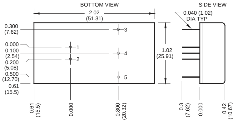
Figure 3. Mechanical Dimensions
