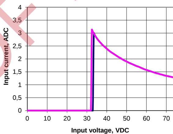
Figure 7. QLS25ZE Input Characteristic
