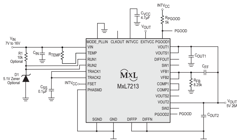
Figure 1: Typical Application: 26A, 5V Output DC/DC Power Module
