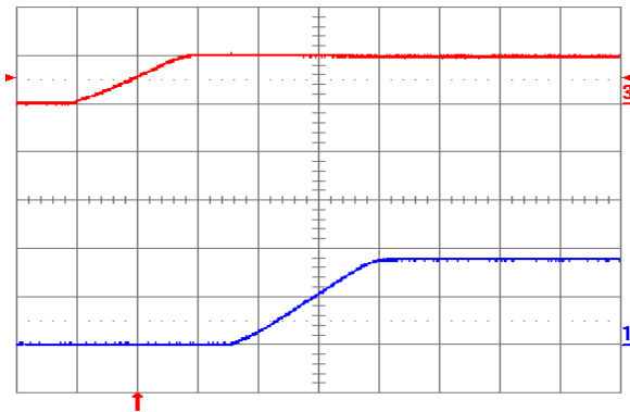
Fig. 1.8V.5: Turn-on transient for V_{out} = 1.8\text{ V} with application of V_{in} at full rated load current (resistive) and 100\mu\text{F} external capacitance at V_{in} = 5\text{ V} . Top trace: V_{in} (5 V/div.); Bottom trace: output voltage (1 V/div.); Time scale: 2 ms/div.
