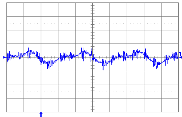
Fig. 2.5V.6: Output voltage ripple (20 mV/div.) at full rated load current into a resistive load with external capacitance 100 \mu\text{F} ceramic + 1 \mu\text{F} ceramic and V_{in} = 5 V for V_{out} = 2.5 V. Time scale: 2 μs/div.
