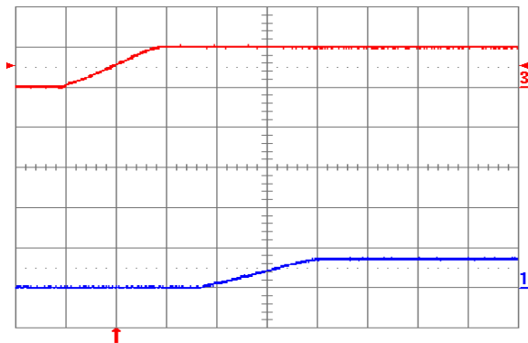
Fig. 0.7525V.5: Turn-on transient for V_{out} = 0.7525 V with application of V_{in} at full rated load current (resistive) and 100 \mu F external capacitance at V_{in} = 5 V. Top trace: V_{in} (5 V/div.); Bottom trace: output voltage (1 V/div.); Time scale: 2 ms/div.
