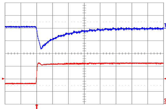
Fig. 1.0V.7: Output voltage response V_{out} = 1.0 V to positive load current step change from 8 A to 16 A with slew rate of 5 A/ \mu s at V_{in} = 5 V. Top trace: output voltage (100 mV/div.); Bottom trace: load current (5 A/div.). C_o = 100 \mu F ceramic + 1 \mu F ceramic. Time scale: 20 \mu s/div.
