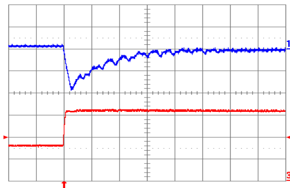
Fig. 3.3V.7: Output voltage for V_{out} = 3.3\text{ V} to positive load current step change from 8 A to 16 A with slew rate of 5\text{ A}/\mu\text{s} at V_{in} = 5\text{ V} . Top trace: output voltage (100 mV/div.); Bottom trace: load current (5 A/div.). C_o = 100\text{ }\mu\text{F} ceramic. Time scale: 20 \mu\text{s} /div.
