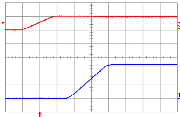
Fig. 2.5V.5: Turn-on transient for V_{out} = 2.5 V with application of V_{in} at full rated load current (resistive) and 100 \mu\text{F} external capacitance at V_{in} = 5 V. Top trace: V_{in} (5 V/div.); Bottom trace: output voltage (1 V/div.); Time scale: 2 ms/div.
