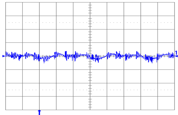
Fig. 0.7525V.6: Output voltage ripple (20 mV/div.) at full rated load current into a resistive load with external capacitance 100 \mu F ceramic + 1 \mu F ceramic and V_{in} = 5 V for V_{out} = 0.7525 V. Time scale: 2 \mu s/div.
