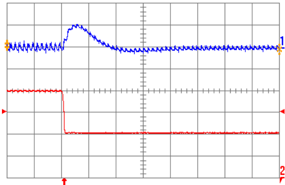
Fig. 2.5V.7: Output voltage response for V_{out} = 2.5 V to negative load current step change from 20 A to 10 A with slew rate of -5A/ \mu s at V_{in} = 12 V. Top trace: output voltage (200 mV/div.); Bottom trace: load current (5 A/div.). C_o = 100 \mu F ceramic. Time scale: 20 \mu s/div.
