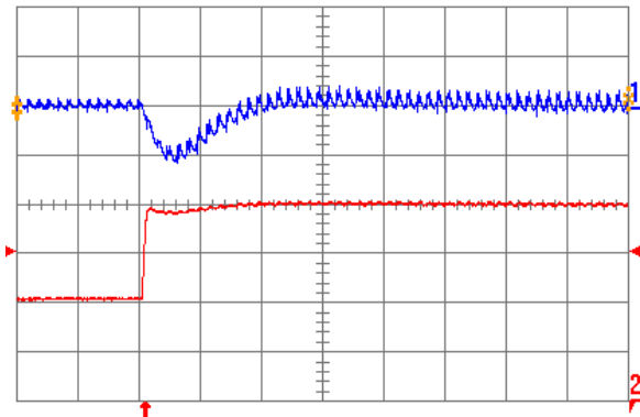
Fig. 2.5V.6: Output voltage response for V_{out} = 2.5 V to positive load current step change from 10 A to 20 A with slew rate of 5A/ \mu s at V_{in} = 12 V. Top trace: output voltage (200 mV/div.); Bottom trace: load current (5 A/div.). C_o = 100 \mu F ceramic. Time scale: 20 \mu s/div.
