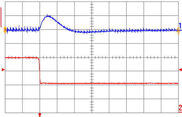
Fig. 1.0V.7: Output voltage response for V_{out} = 1.0 V to negative load current step change from 20 A to 10 A with slew rate of -5\text{ A}/\mu\text{s} at V_{in} = 12 V. Top trace: output voltage (200 mV/div.); Bottom trace: load current (5 A/div.). C_o = 100 \mu\text{F} ceramic. Time scale: 20 \mu\text{s} /div.
