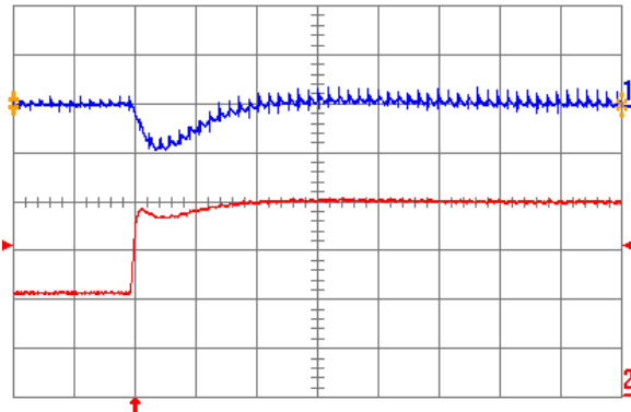
Fig. 1.0V.6: Output voltage response for V_{out} = 1.0 V to positive load current step change from 10 A to 20 A with slew rate of 5\text{ A}/\mu\text{s} at V_{in} = 12 V. Top trace: output voltage (200 mV/div.); Bottom trace: load current (5 A/div.). C_o = 100 \mu\text{F} ceramic. Time scale: 20 \mu\text{s} /div.
