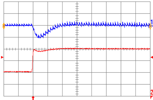
Fig. 1.5V.6: Output voltage response for V_{out} = 1.5\text{ V} to positive load current step change from 10 A to 20 A with slew rate of 5\text{ A}/\mu\text{s} at V_{in} = 12\text{ V} . Top trace: output voltage (200 mV/div.); Bottom trace: load current (5 A/div.). C_o = 100\text{ }\mu\text{F} ceramic. Time scale: 20 µs/div.
