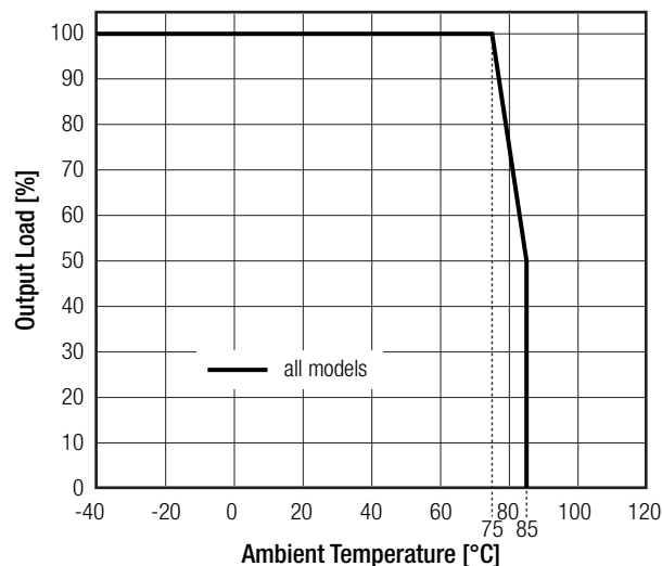
@ 140-305VAC
