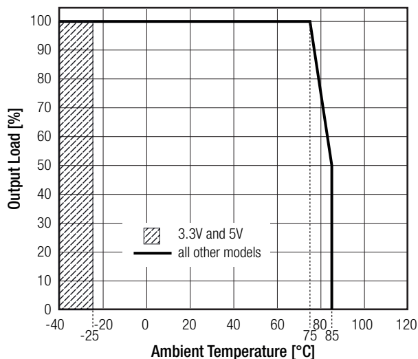
@ 85-140VAC
