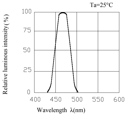
Spectrum Distribution
