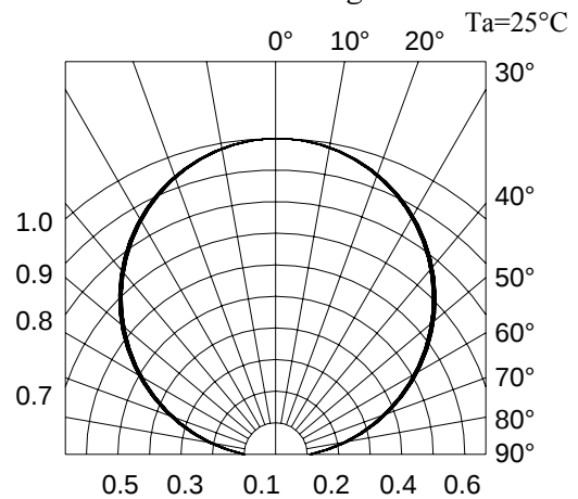
Radiation Diagram
