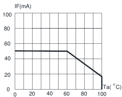
FIG.5 MAXIMUM FORWARD DC CURRENT VS AMBIENT TEMPERATURE ( T_{jmax}=110^{\circ}\text{C} )
