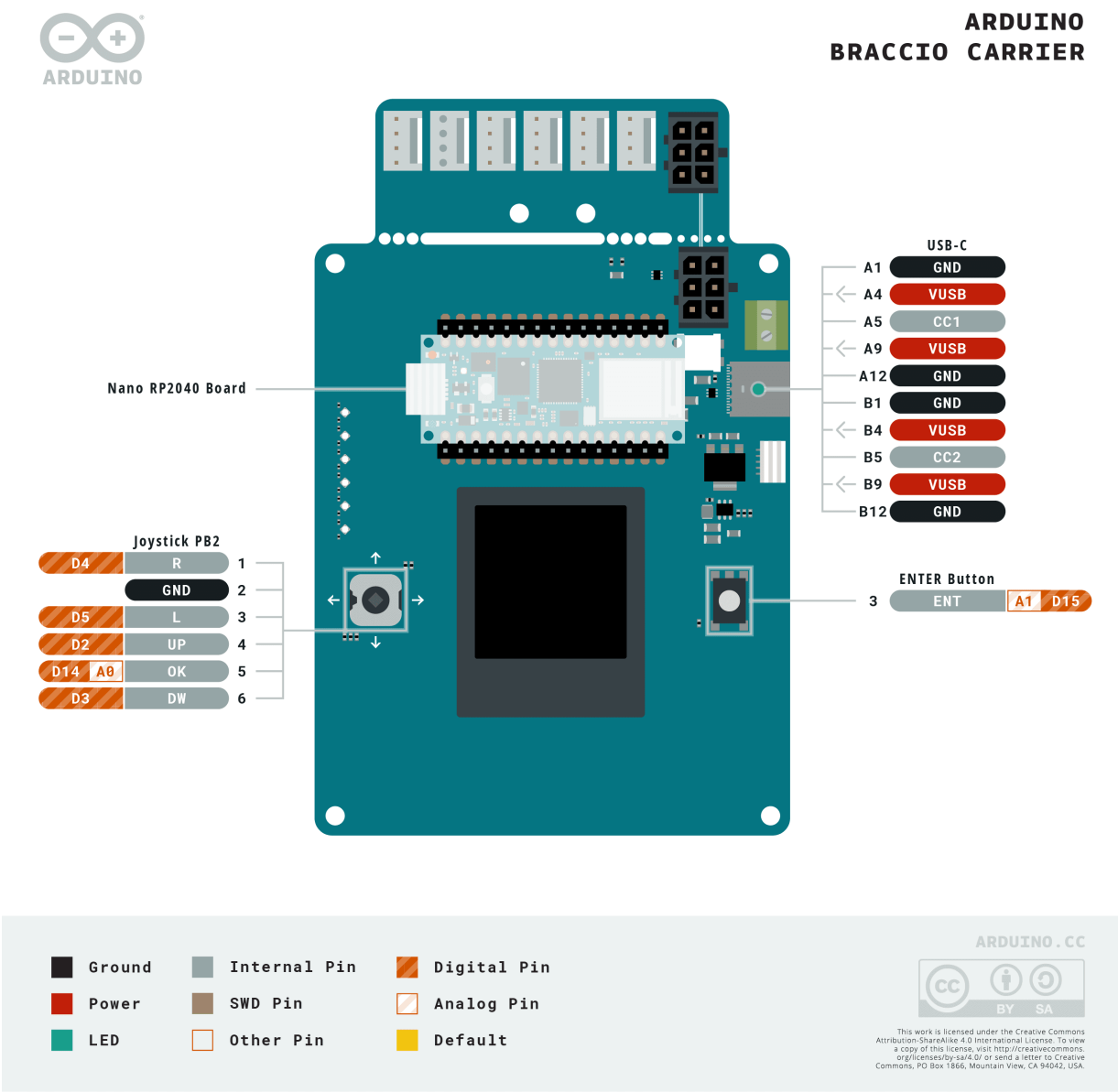
Braccio Carrier Pinout
