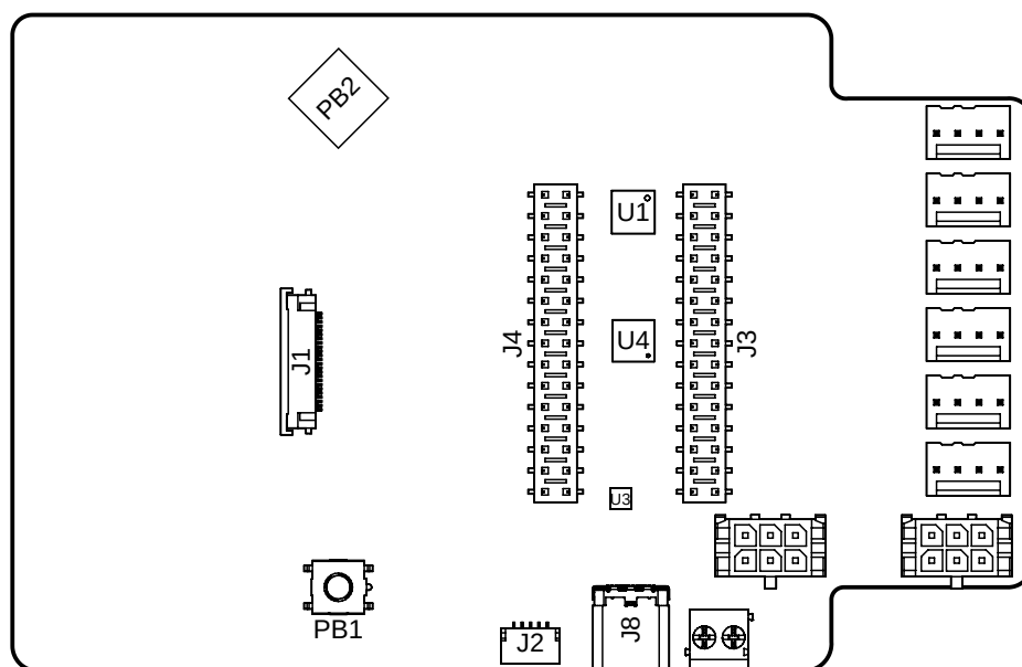
4.2 Board Topology
