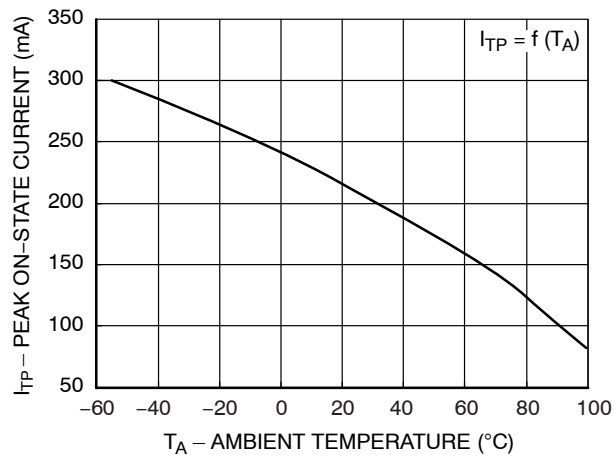
Figure 11. Current Reduction
