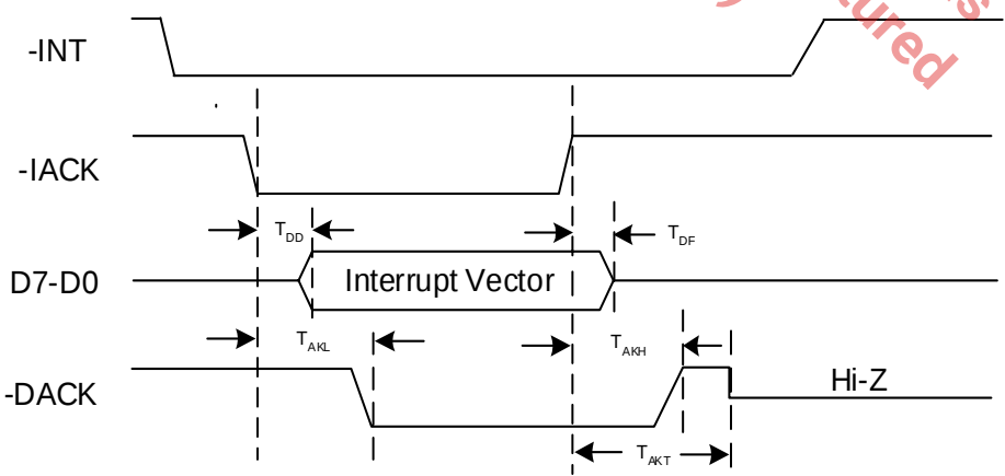
Figure 7: Interrupt Timing
