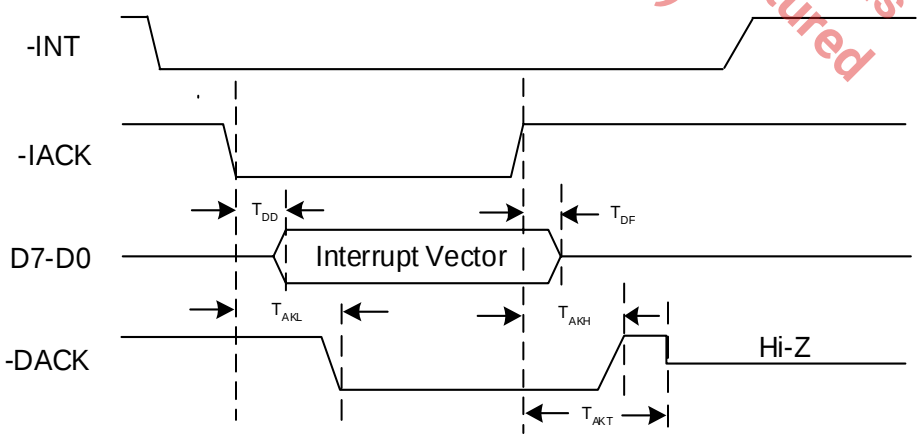
Figure 7: Interrupt Timing
